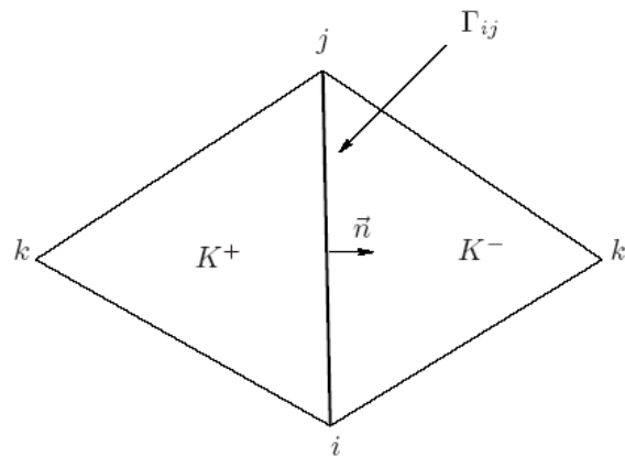
Figure 1: Geometrical elements for defining the scheme.
