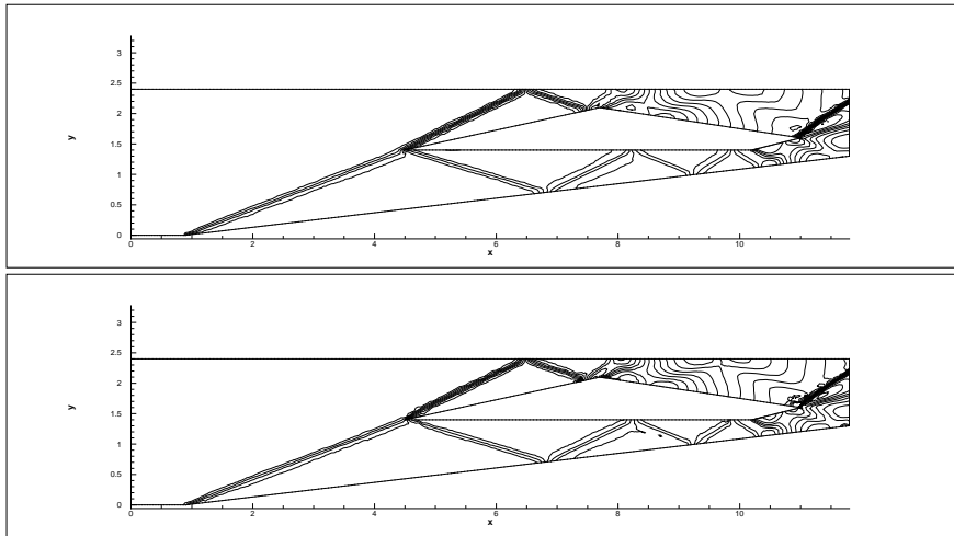
Figure 6: Mach number for the "classical" scheme continuous elements and the scheme discontinuous element described in this paper. 20 isolines are represented.
