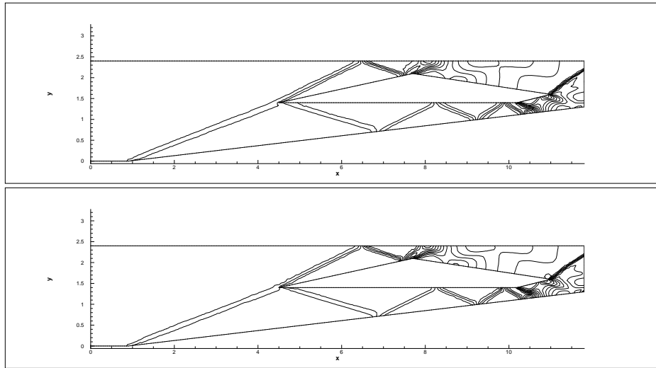
Figure 4: Density isolines for the "classical" scheme continuous elements and the scheme discontinuous element described in this paper. 30 isolines are represented.
