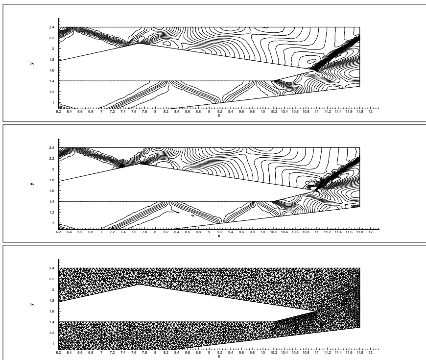
Zoom of the mesh, exit zone.
