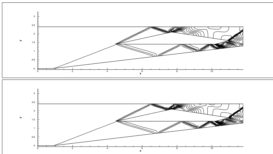
Figure 5: Pressure field for the "classical" scheme continuous elements and the scheme discontinuous element described in this paper. 30 isolines are represented.
