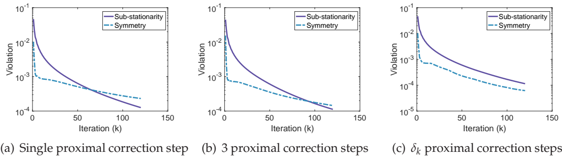
Figure 1: Comparison of multiple proximal correction steps.
