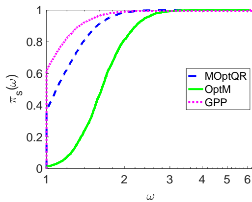
Figure 9: Performance profile on 2304 problems with respect to CPU time.
