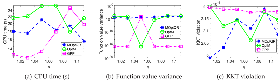
Figure 7: Comparison of GPP, OptM and MOptQR for different \eta on Problem 2.
