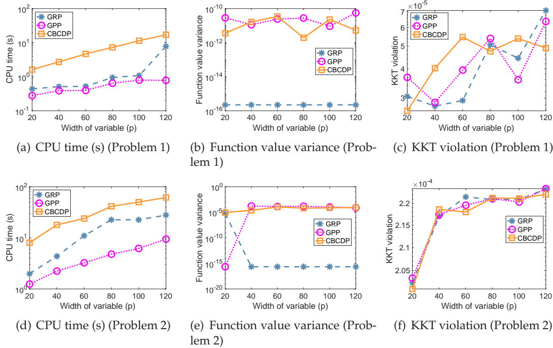
Figure 3: Comparison of GRP, GPP, and CBCDP for different p .
