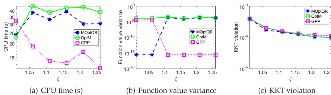
Figure 8: Comparison of GPP, OptM and MOptQR for different \zeta on Problem 2.
