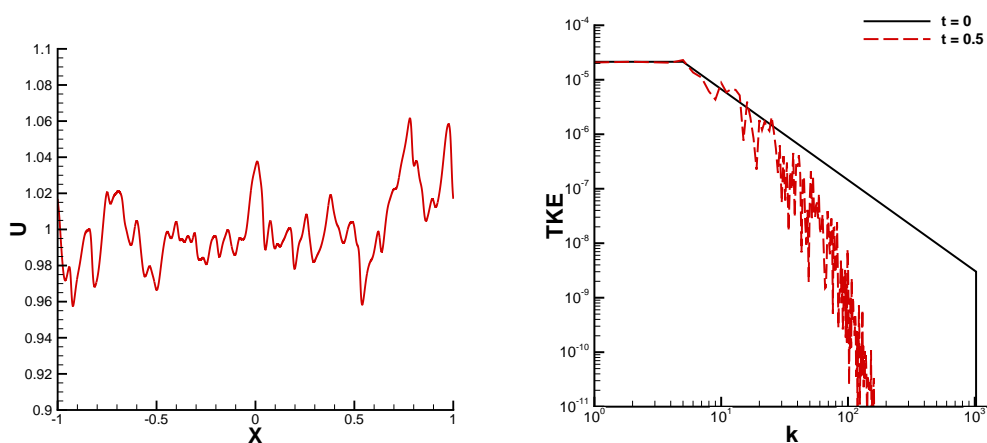
Figure 3: The solution and its spectrum of the DNS solution at t=0.5 .
