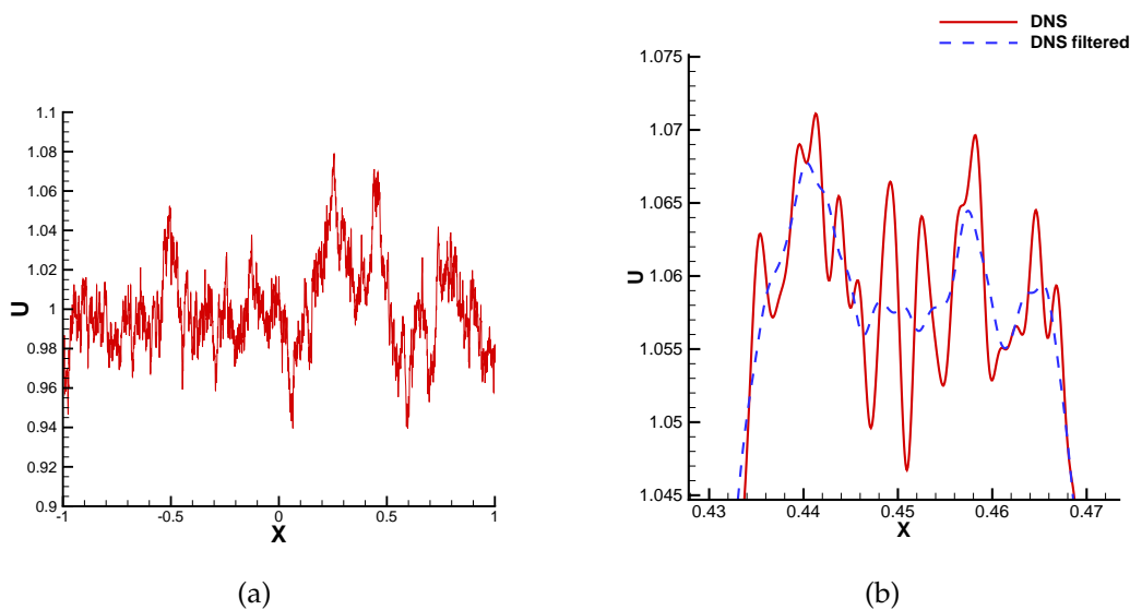
Figure 2: One realization of the initial condition and the filtered solution.
