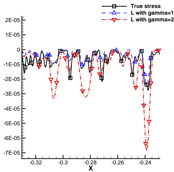
Figure 6: Comparison between the true stress computed with the sub-grid-scale between k_\Delta and 2k_\Delta and the modelled stresses computed using \hat{u} .
