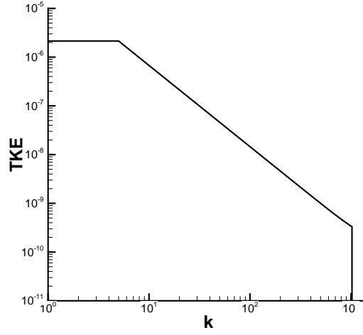
Figure 1: The initial energy spectrum.
