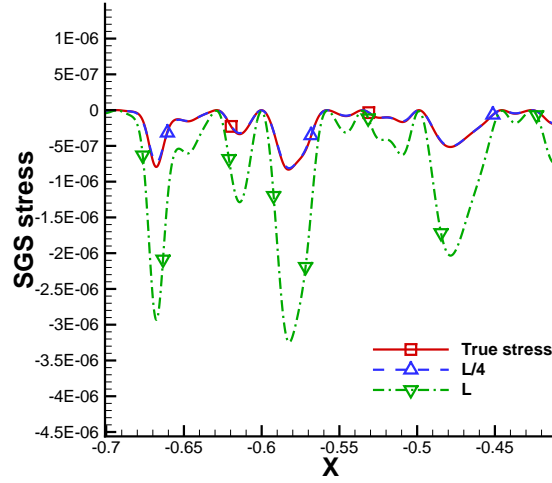
Figure 4: Comparison of the true stress and the modeled stress based on the SSM of Bardina. When we first saw the relation (1.9), we suspected that this was a bug. After we tested different initial conditions, we were convinced that it was not a bug. The fact that (1.9) is true for arbitrarily-generated random initial conditions prompted us to look for a deeper reason resulting in the following analysis.
