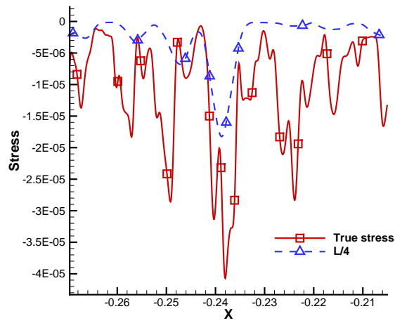
Figure 5: The true stress and the modeled stress for the full spectrum given in Fig. 1.
