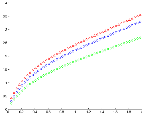
Figure 13: Circulation vs. formation time - numerical results, for AR = 1 , triangles - 50% span, circles - 75% span, diamonds - 90% span.
