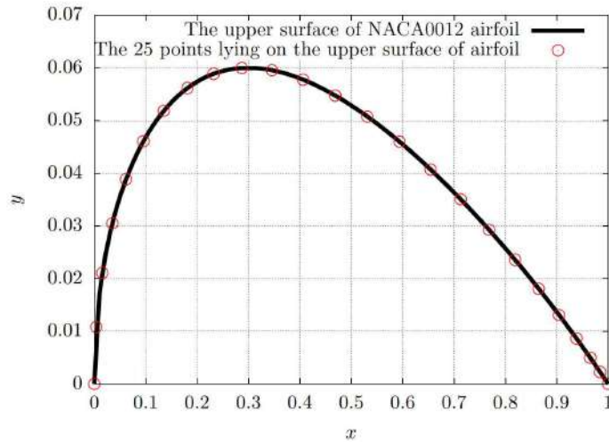
Figure 3: The upper surface of NACA0012 airfoil, and the distribution of points on it.
