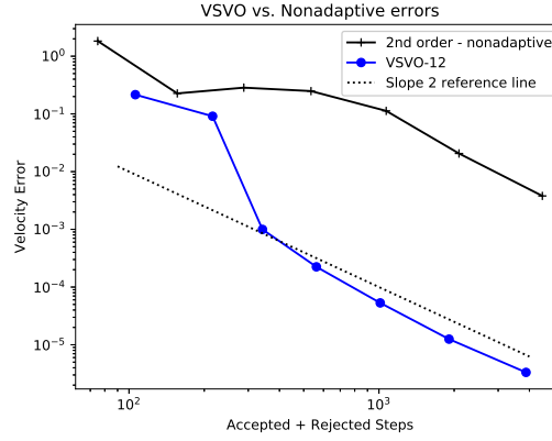
FIGURE 4. The VSVO-12 method performs three orders of magnitude better for the same amount of work compared to the nonadaptive 2nd order method for the test problem in Section 6.2. Each circle represents a different tolerance from TOL = 10^{-1} to 10^{-7} .
