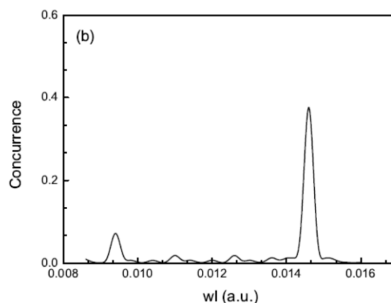
Figure 2: The mean values of the concurrence over long time T for initial state |0, 2\rangle as a function of laser frequency
