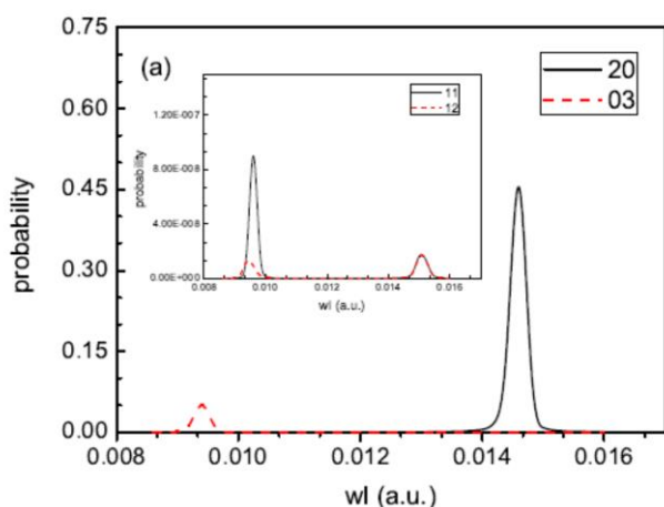
Figure 1: The long-time-averaged probability as a function of laser frequency
