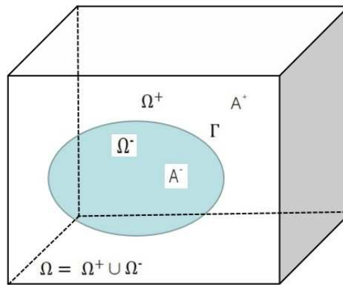
Fig. 1.1. A diagram of the anisotropic interface problem: a rectangular domain with a closed smooth interface (surface).
