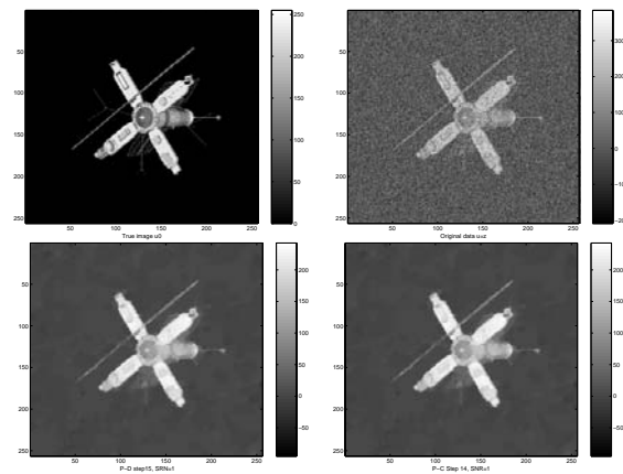
Figure 3 (Satellite) Top left is original image and top right is noise image. \alpha = 50, \beta = 10^{-20}, tol = 10^{-4} . Bottom left is from P-D and bottom right from P-C.
