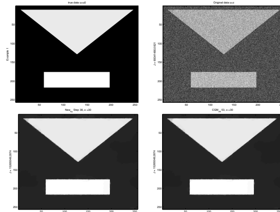
Figure 1 Top left is original image and top right is noise image. \alpha = 30, \beta = 10^{-20}, tol = 10^{-4} . Bottom left is from P-D and bottom right from P-C.
