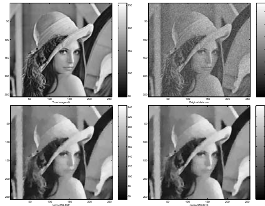
Figure 2 (Lenna) Top left is original image and top right is noise image. \alpha = 30, \beta = 10^{-20}, tol = 10^{-4} . Bottom left is from P-D and bottom right from P-C.
