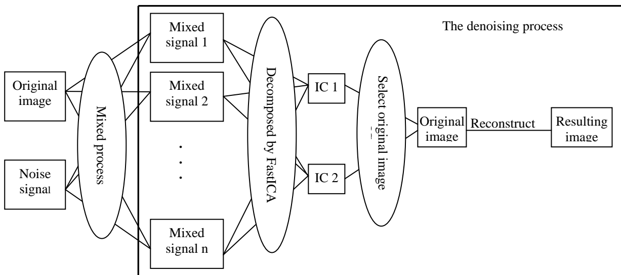
Fig. 2 Process of noise separation in MCIs based on FastICA
