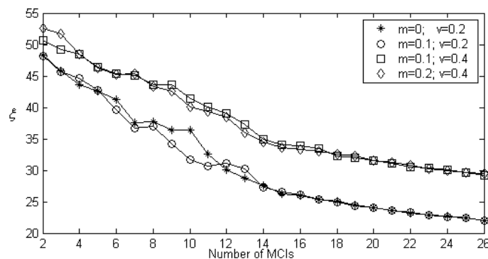
Fig. 5 Influence of the number of MCIs upon the denoising result.
