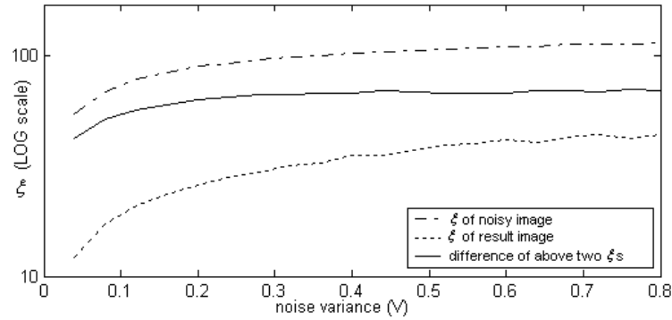
Fig. 6 Influence of the noise variance upon the denoising result with the noise mean M = 0.1 ; the number of MCIs is set to 14.
