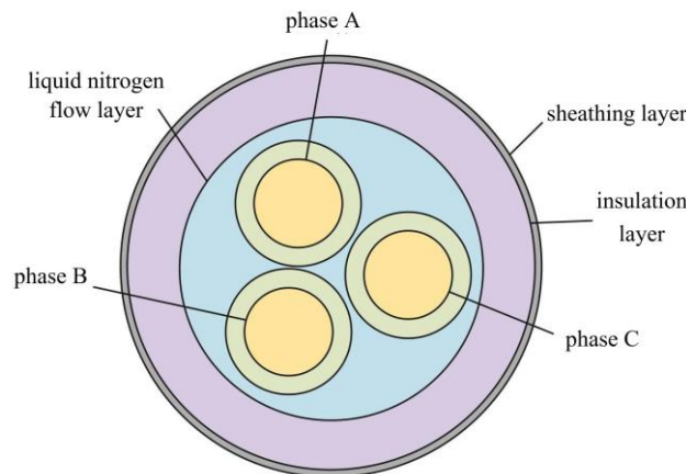
Figure 2: Cable section diagram
