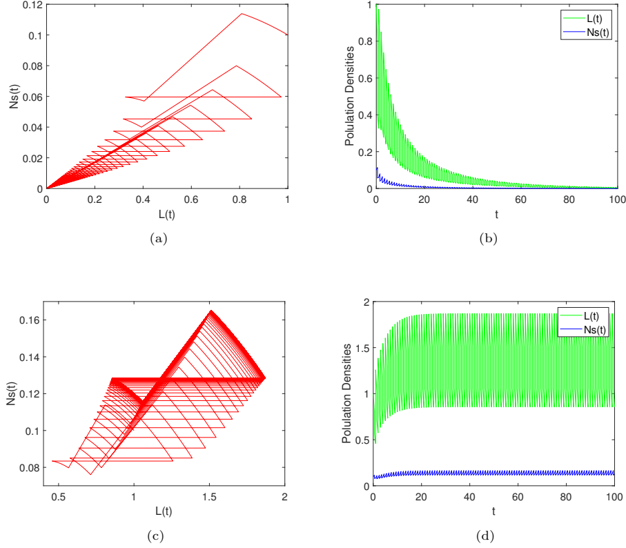
Figure 1. The phase portrait(a) and time-series diagram(b) of trivial periodic solution (0, 0) of system (4.2) with initial conditions L_0 = 1, N_0^S = 0.1 and q = 0.5 ; the phase portrait(c) and time-series diagram(d) of nontrivial periodic solution (L^*, N^*) of system (4.2) with q = 0.3 .
