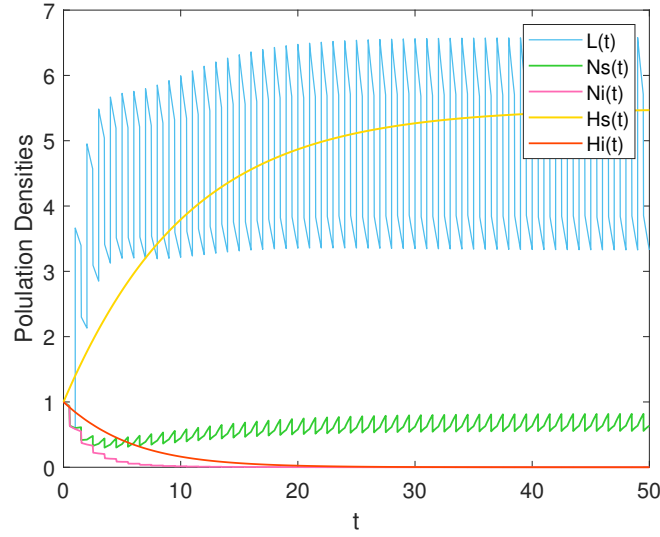
Figure 2. The time-series diagram of globally attractive disease-free periodic solution (\widetilde{L}_t, \widetilde{N}_t, 0, \overline{H}, 0) to system (2.1) with initial conditions (1, 1, 1, 1, 1) and the following parameter values T = 1 , l = 0.5 , q = 0.32 , r = 200 , w = 50 , \beta^L = 0.045 , \eta^L = 0.4 , \eta^N = 0.5 , \beta^N = 0.05 , p^N = 0.4 , \mu^T = 0.05 , \Lambda = 0.55 , p^H = 0.6 , \mu^H = 0.1 , \alpha^H = 0.1 .
