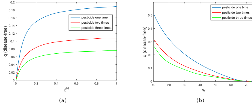
Figure 4. The minimum intensity of the sprayed pesticide that makes the disease disappear with respect to different parameters: (a) nymphal biting rate \beta^N and (b) adult density-dependent rate w .
