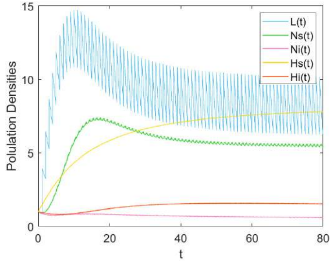
Figure 3. The time-series diagram of disease persistent periodic solution to system (2.1) with initial conditions (1, 1, 1, 1, 1) and the following parameter values T = 1 , l = 0.5 , q = 0.02 , r = 200 , w = 50 , \beta^L = 0.045 , \eta^L = 0.8 , \eta^N = 0.7 , \beta^N = 0.04 , p^N = 0.6 , \mu^T = 0.05 , \Lambda = 0.55 , p^H = 0.8 , \mu^H = 0.05 , \alpha^H = 0.05 .
