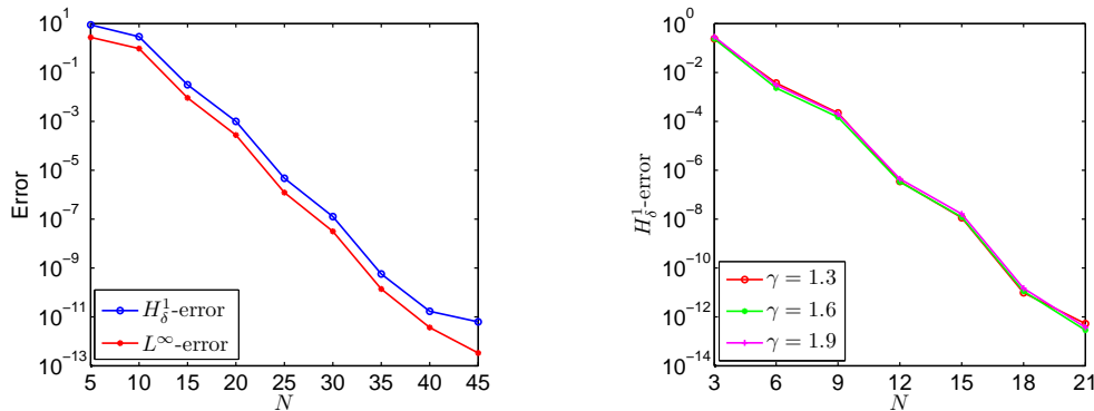
Figure 6: Left: L^\infty -errors and H_\delta^1 -errors against N in semi-log scale (Example 4.5); Right: H_\delta^1 -errors against N in semi-log scale (Example 4.6).
