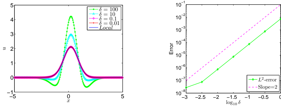
Figure 2: Left: Numerical solutions of nonlocal and local models; Right: L^2 -errors against \delta in log-log scale.
