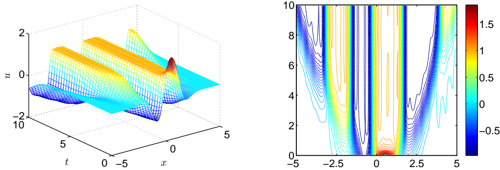
Figure 8: Time evolutions of the nonlocal numerical solution for \delta = 0.1 . Left: the mesh plot; Right: the contour.
