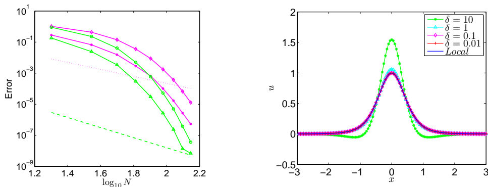
Figure 3: Left: L^\infty -errors ( \bullet for h = 3 and \triangle for h = 4 ) and H_\delta^1 -errors ( \diamond for h = 3 and \circ for h = 4 ) against N in log-log scale; Right: numerical solutions of nonlocal and local models. The dotted line with the slope -\frac{9}{4} and the dashed line with the slope -\frac{13}{4} are used on the left side for reference.
