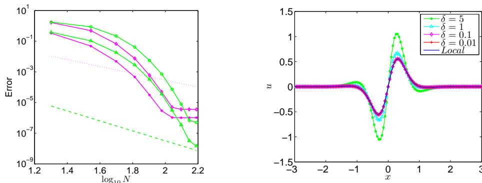
Figure 4: Left: L^\infty -errors ( \bullet for h = 3 and \triangle for h = 4 ) and H_\delta^1 -errors ( \diamond for h = 3 and \circ for h = 4 ) against N in log-log scale; Right: numerical solutions of nonlocal and local models. The dotted line with the slope -\frac{9}{4} and the dashed line with the slope -\frac{13}{4} are used on the left side for reference.
