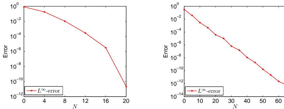
Figure 9: L^\infty -errors against N in semi-log scale. Left: u(x) = e^{-(x_1^2+x_2^2)/2}(1-x_1^2/10)^4(1+x_1^2/10)^6 ; Right: u(x) = e^{-(x_1^2+x_2^2)/2} \sin(x_1 x_2) .
