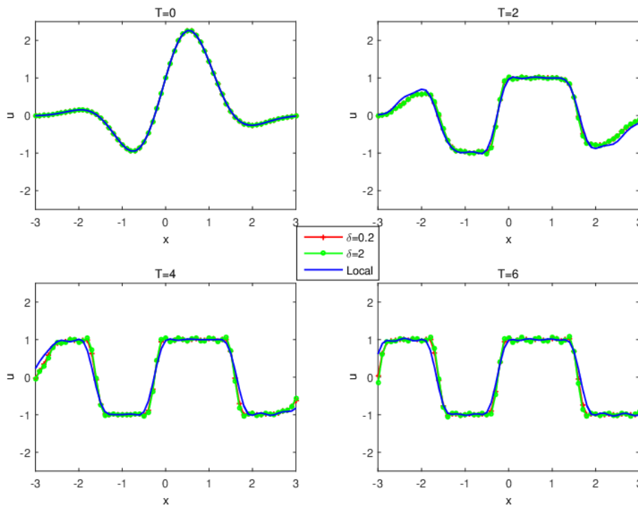
Figure 7: Snapshots of numerical solutions for both local and nonlocal Allen-Cahn equations at different time with \delta = 2, 0.2 .
