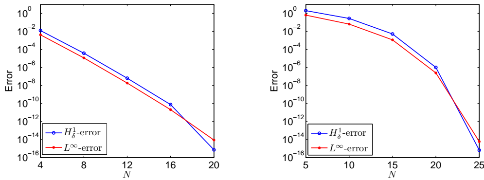
Figure 1: L^\infty -errors and H_\delta^1 -errors against N in semi-log scale. Left: fixed \alpha ; Right: adaptive \alpha_N .
