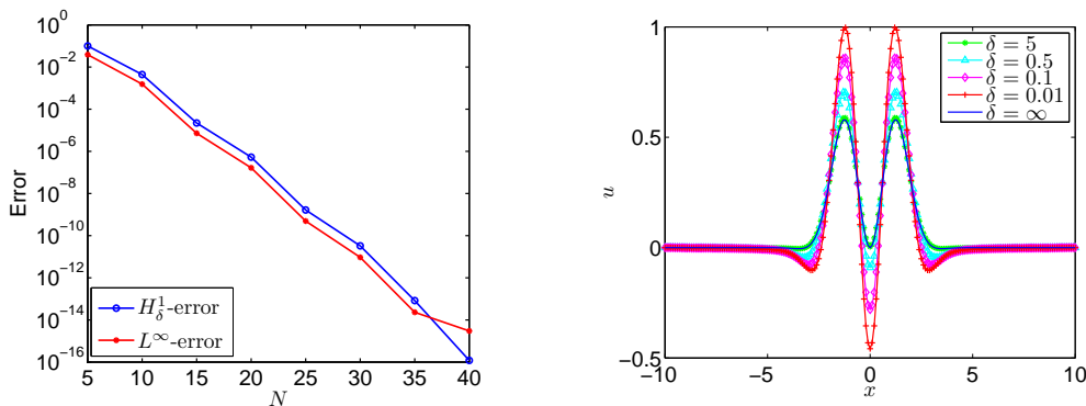
Figure 5: Left: L^\infty -errors and H_\delta^1 -errors against N in semi-log scale; Right: numerical solutions of truncated and usual models.
