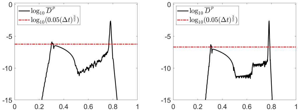
Figure 4: Example 5.2: \log_{10} \bar{D}^p and \log_{10}(0.05(\Delta t)^{3/2}) for \Delta x = 1/400 (left) and 1/800 (right).
