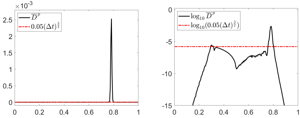
Figure 3: Example 5.2: \bar{D}^p and 0.05(\Delta t)^{3/2} (left) and \log_{10} \bar{D}^p and \log_{10}(0.05(\Delta t)^{3/2}) (right) for \Delta x = 1/200 .
