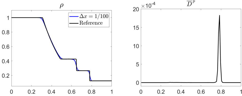
Figure 1: Density (left) and the corresponding values of the pressure-based LSI (right).
