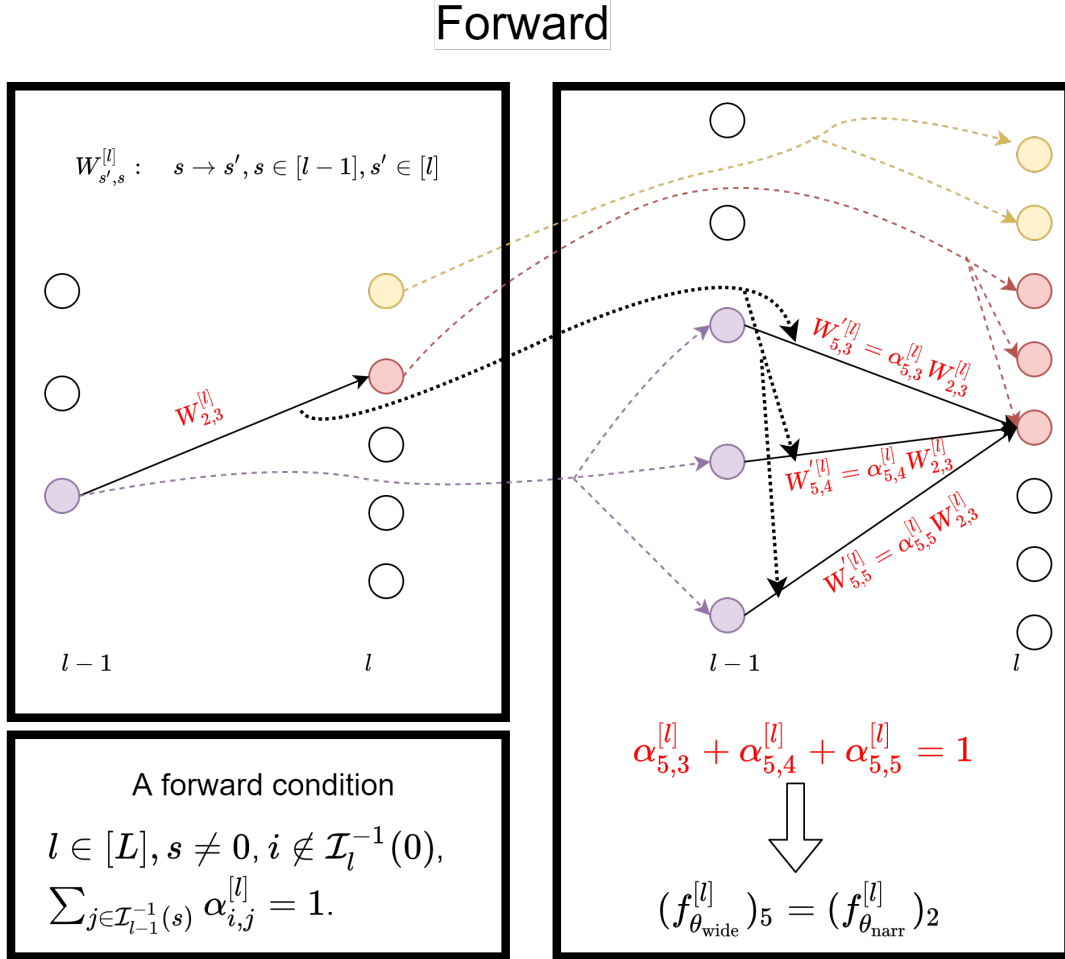
Figure 7: Illustration of the forward conditions for split neurons in compatibility conditions I. The sum of the input weights from neurons that are split from the same previous neuron to a post neuron should be equal to the weight from the previous to the post neuron.
