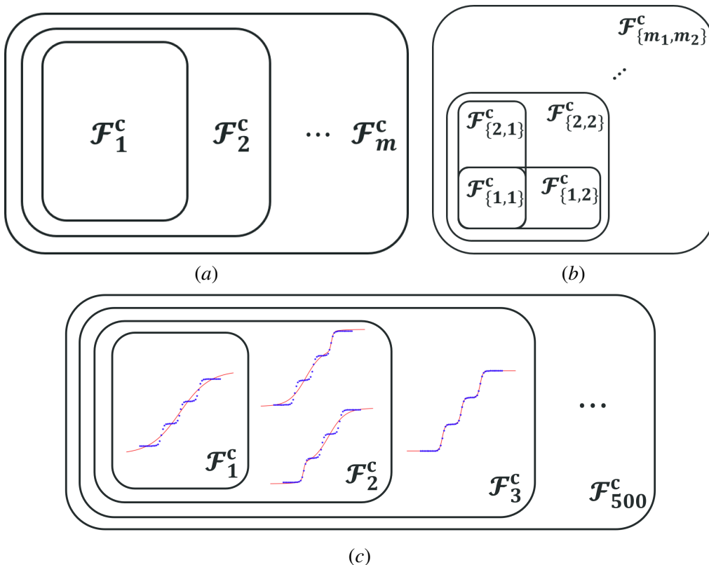
Figure 4: Illustration of the Embedding Principle for the critical functions of (a) two-layer width- m NN and (b) three-layer width- \{m_1, m_2\} NN. (c) Some critical functions of width-500 tanh-NN predicted by the Embedding Principle for experiments in Fig. 3.
