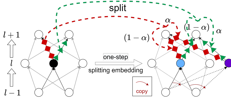
Figure 2: Illustration of one-step splitting embedding. The black neuron in the left network is split into the blue and purple neurons in the right network. The red (green) output weight of the black neuron in the left net is split into two red (green) weights in the right net with ratio (1 - \alpha) and \alpha , respectively. This is also illustrated in Zhang et al. (2021b).
