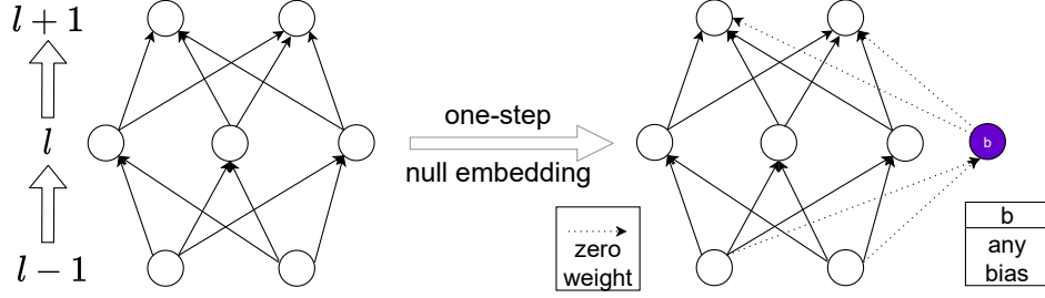
Figure 1: Illustration of one-step null embedding. The purple neuron is added with both input and output weights as zero and an arbitrary bias.
