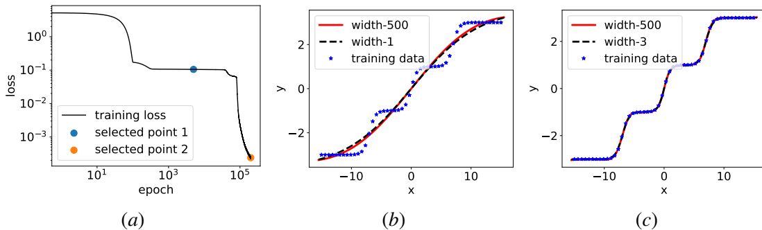
Figure 3: (a) The training loss of a two-layer tanh neural network with 500 hidden neurons. (b, c) Red solid: the DNN output at a training step, where the blue dot and the orange dot in (a) corresponds to (b) and (c), respectively; Black dashed: the output of the global minimum of the width-1 NN in (b) and the width-3 NN in (c), respectively; Blue dots: training data. This is also illustrated in Zhang et al. (2021b)
