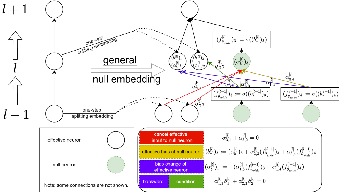
Figure 9: Illustration of compatibility conditions for null neurons. Red: The input from effective neurons split from the same neuron should cancel out. Yellow: the effective bias of a null neuron is the sum of its bias (can be any value) and its input from other null neurons. Purple: The added null neurons have constant input to the effective neuron, which would be added a bias correction to cancel the constant input. Purple+Green: the backward condition of a null neuron leads to the zero gradient.
