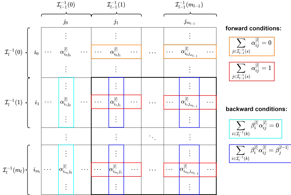
Figure 5: Illustration of forward and backward compatibility conditions I for \alpha^{[l]} .
