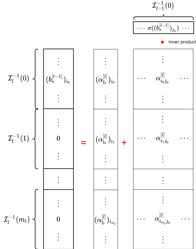
Figure 6: Illustration of compatibility conditions II for \alpha_{\mathbf{b}}^{[l]} .
