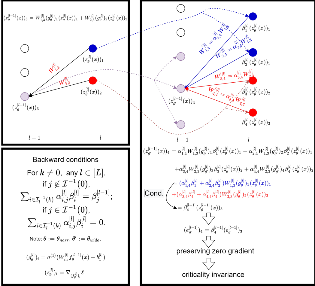
Figure 8: Illustration of the backward conditions for split neurons in compatibility conditions I. The gradient of the loss w.r.t. to the neuron output of the wide network is proportional to the gradient of the loss w.r.t. the corresponding neuron in the narrow network.
